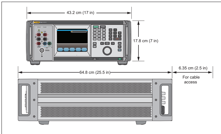
Figure 1. Product Dimension
